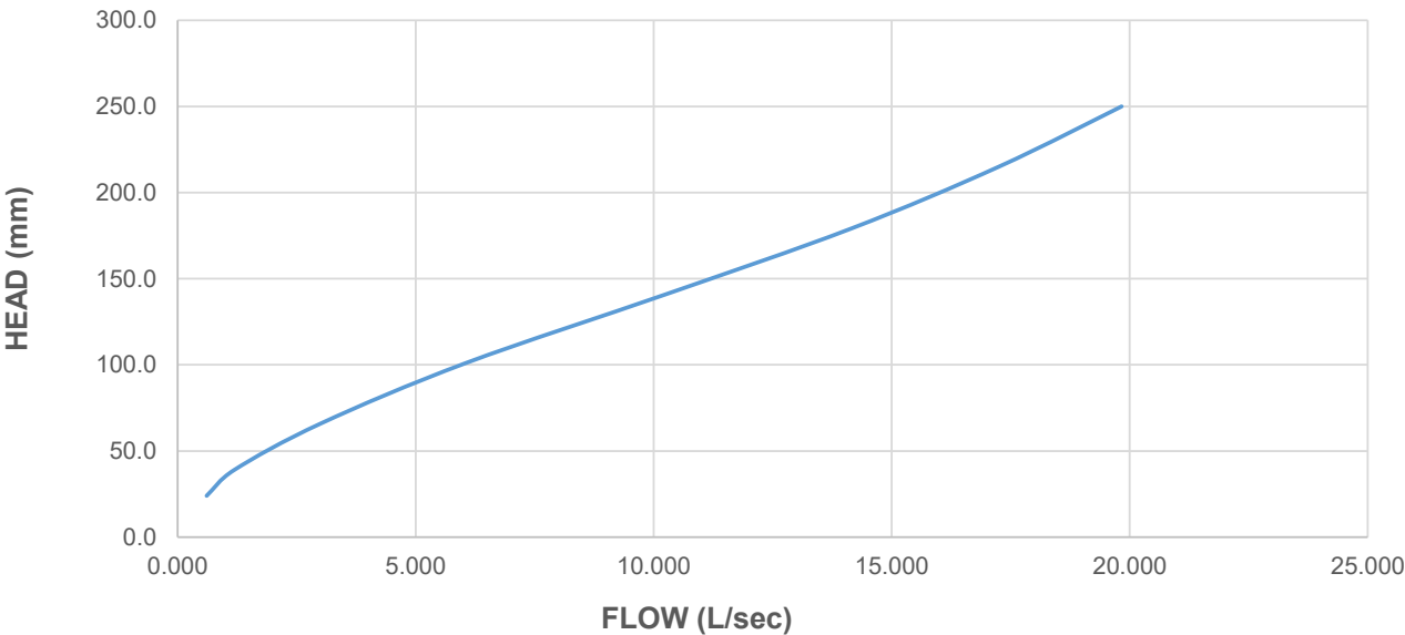
Flow Characteristic Curve for: 2200.712 Scupper 150 Round with Scupper Guard Condition: Fitting only
