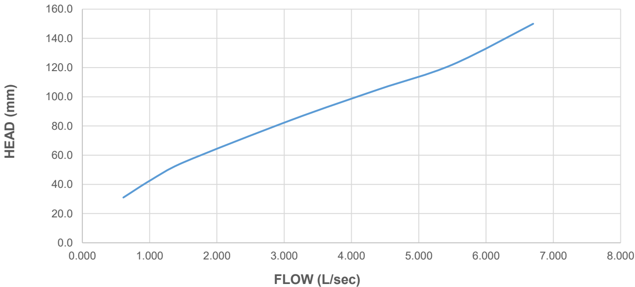
Flow Characteristic Curve for: 2200.612 Scupper 100 Round with Scupper Guard Condition: Fitting only
