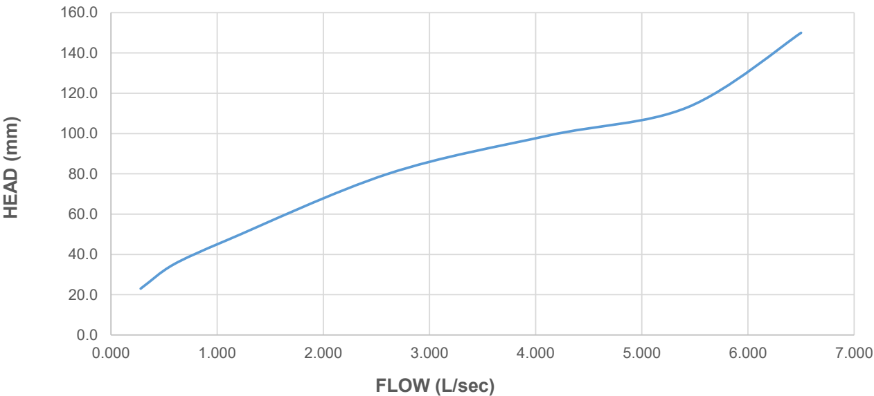
Flow Characteristic Curve for: 2200.512 Scupper 80 Round with Scupper Guard Condition: Fitting only
