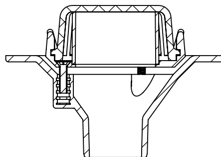
SECTION BU-BU 3100.173.2 configured for overflow
