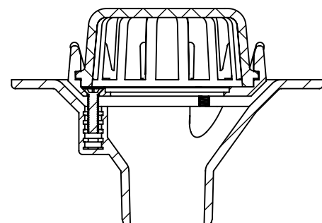
SECTION BT-BT 3100.173.2 configured for drain
