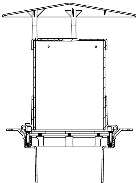
SECTION F-F
