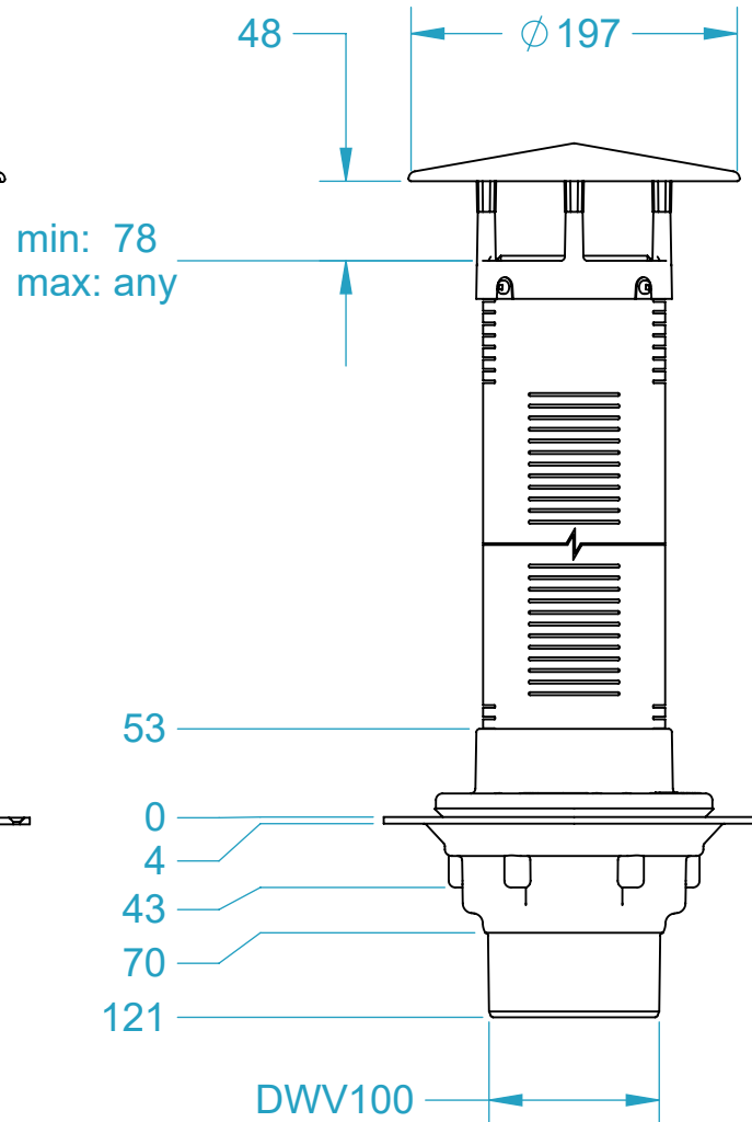
SECTION E-E
