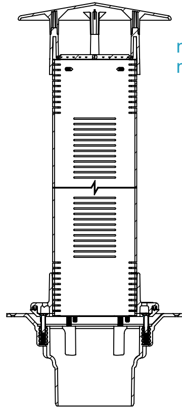
SECTION E-E
