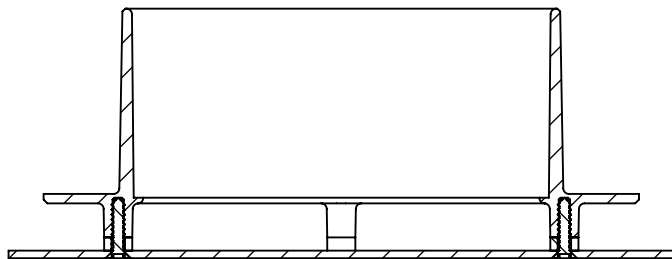
SECTION F-F
