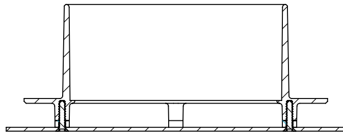
SECTION E-E
