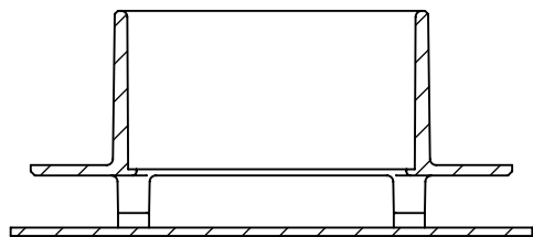
SECTION E-E
