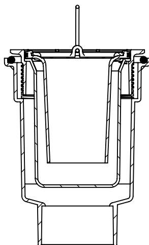
SECTION Z-Z
