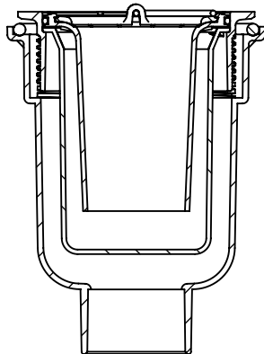
SECTION H-H
