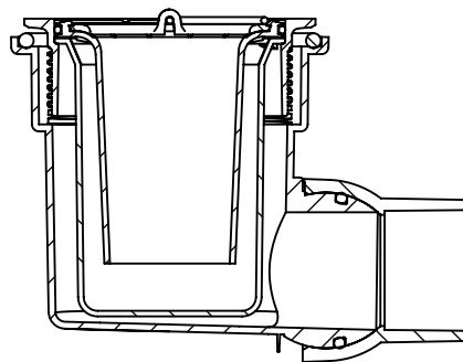
SECTION G-G
