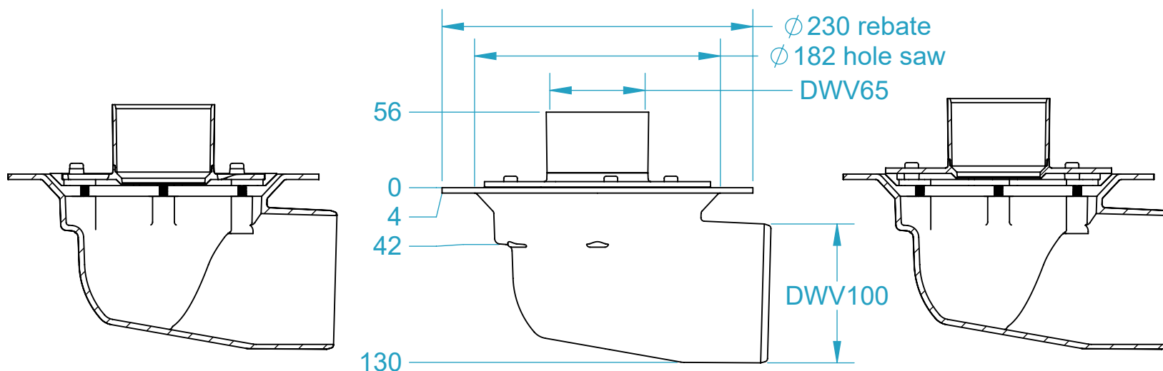
SECTION AB-AB
