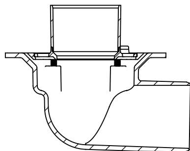
SECTION T-T
