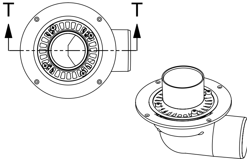
3000.111.4 Vented
