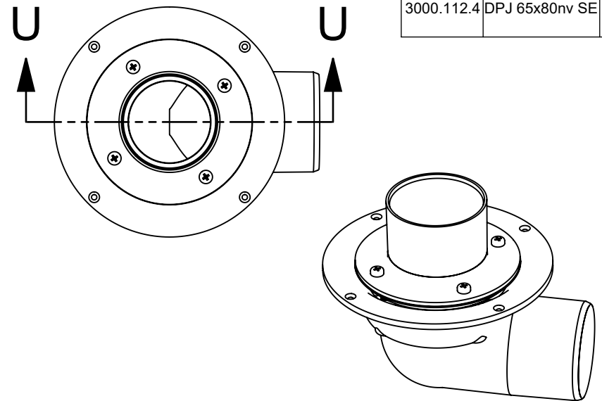
3000.112.4 Non-Vented
