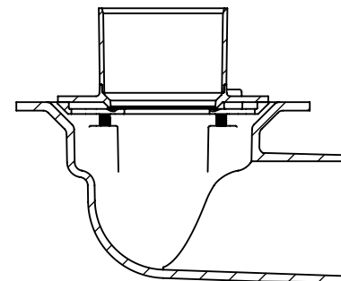
SECTION U-U
