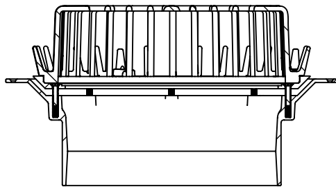
SECTION R-R 3100.405.SS configured for drain
