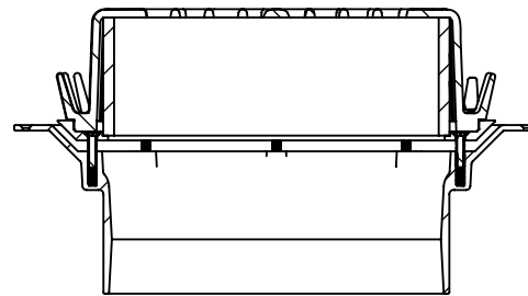
SECTION K-K 3100.405.SS configured for overflow
