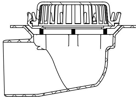
SECTION P-P 3100.207 configured for drain
