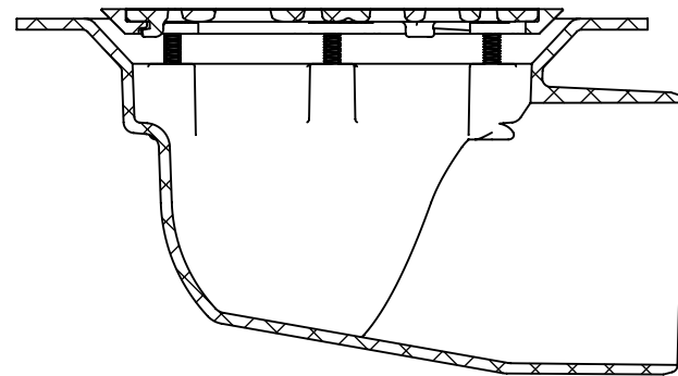
SECTION N-N
