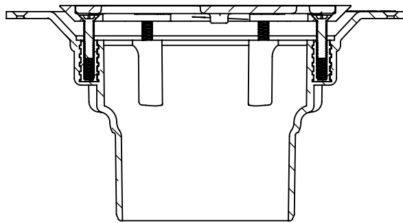
SECTION M-M
