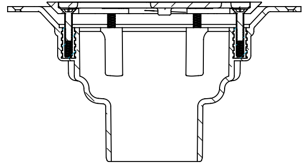
SECTION G-G
