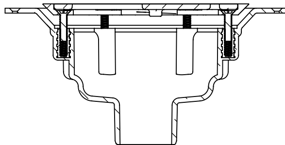
SECTION F-F
