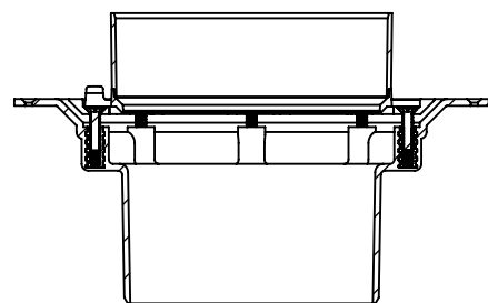
SECTION T-T
