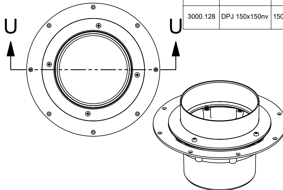
3000.128 Non-Vented
