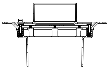
SECTION P-P
