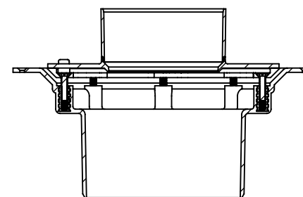
SECTION R-R
