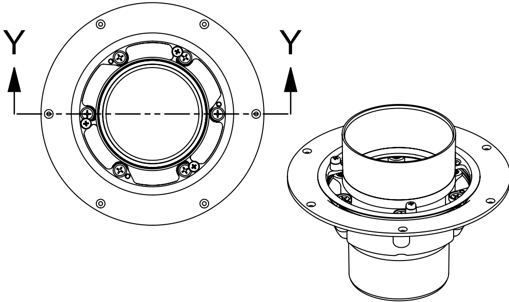
3000.123 Vented
