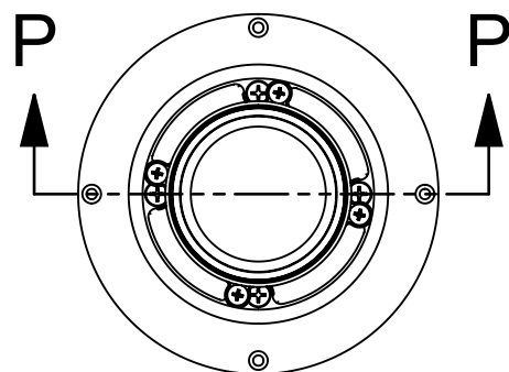
3000.117 Vented
