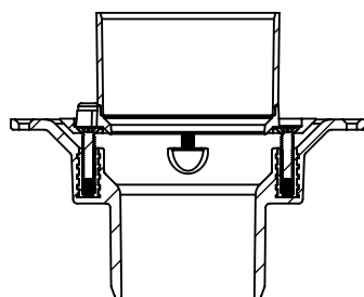
SECTION P-P
