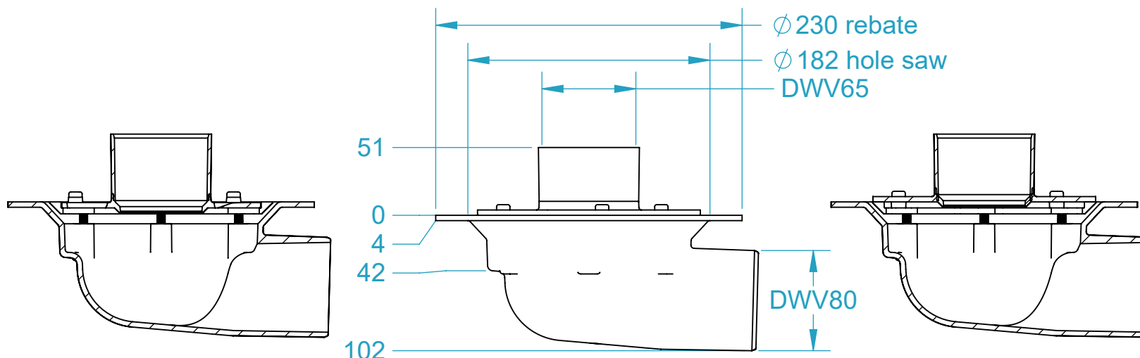
SECTION AH-AH
