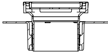
SECTION C-C
