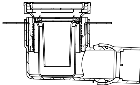
SECTION L-L
