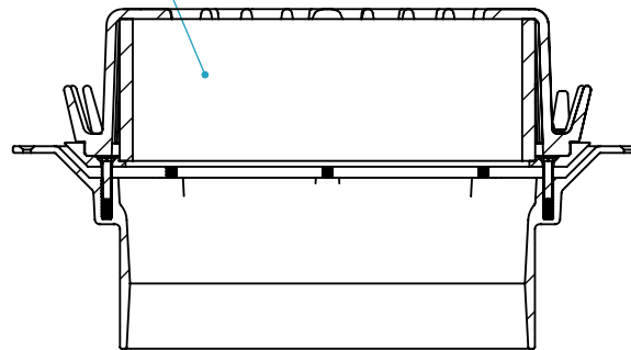
OVERFLOW SECTION
