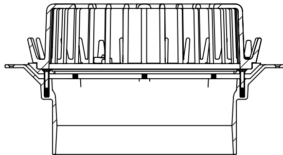
ROOF DRAIN SECTION
