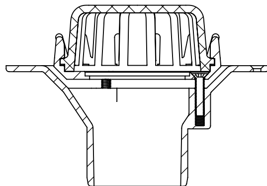
ROOF DRAIN SECTION
