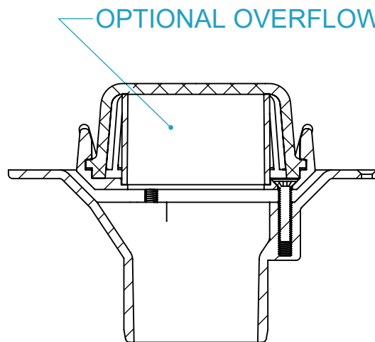
OVERFLOW SECTION
