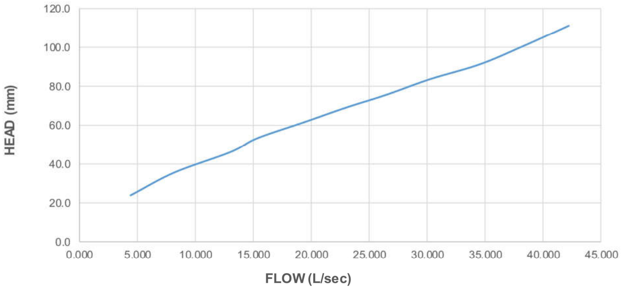
Flow Characteristic Curve for: Roof Drain 225mm Condition: Fitting only
