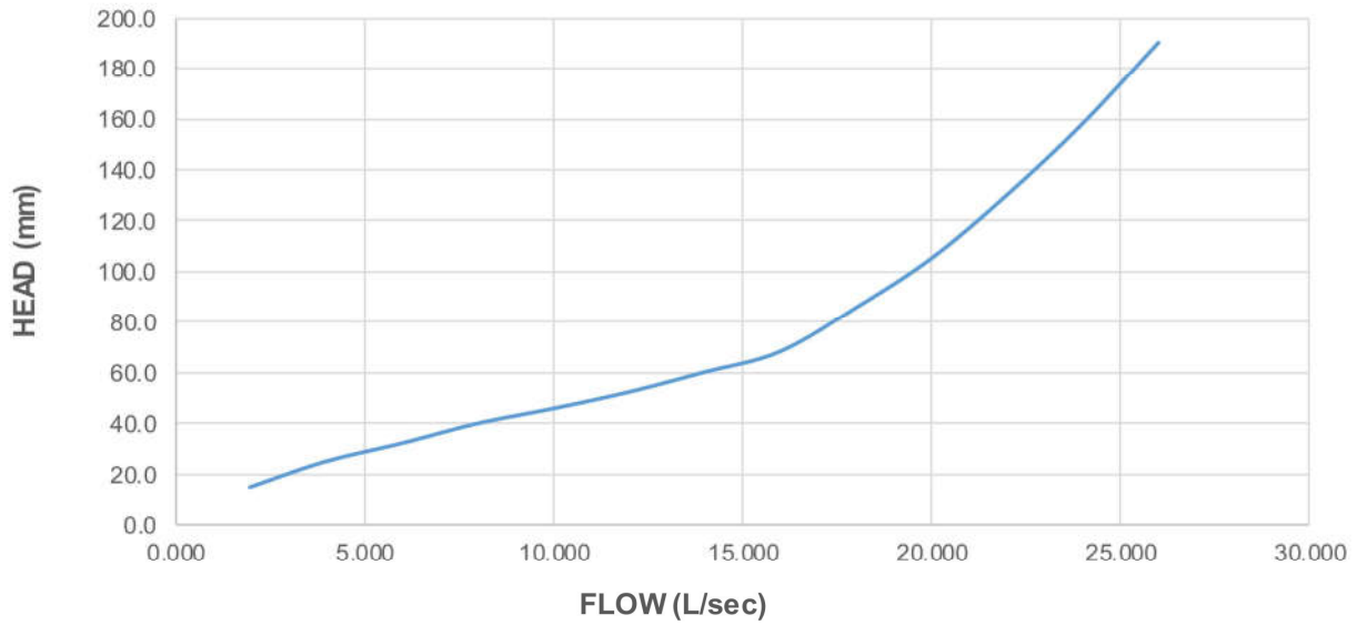
Flow Characteristic Curve for: Roof Drain 150mm Condition: Fitting only
