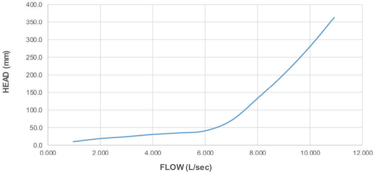
Flow Characteristic Curve for: Roof Drain 80mm Condition: Fitting only
