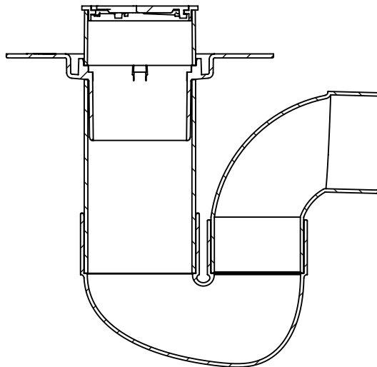
SECTION H-H SCALE 1 : 4
