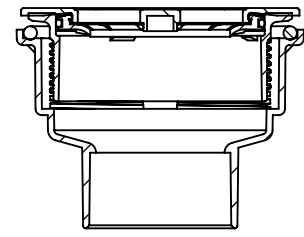
SECTION O-O
