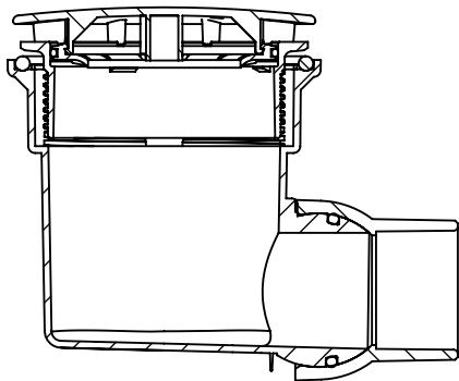
SECTION R-R
