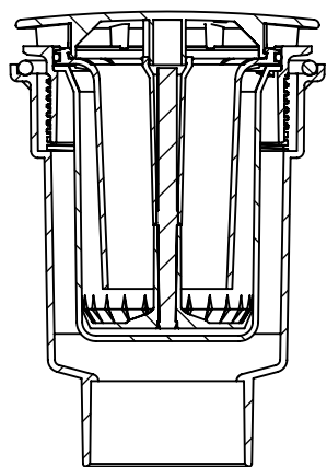
SECTION I-I
