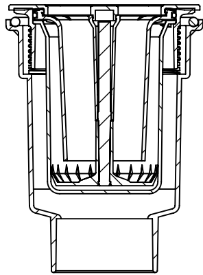
SECTION H-H
