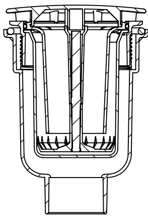
SECTION J-J
