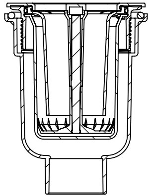
SECTION K-K
