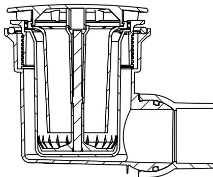
SECTION F-F
