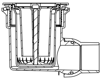
SECTION G-G
