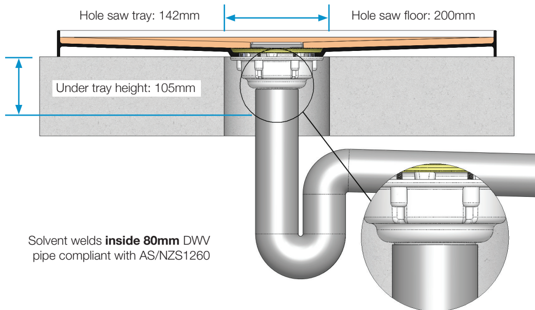
Stainless Lid 1000.191
